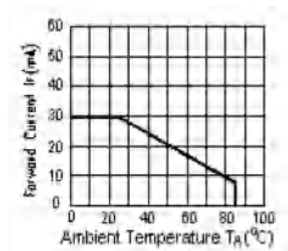
I LED VS TEMP
